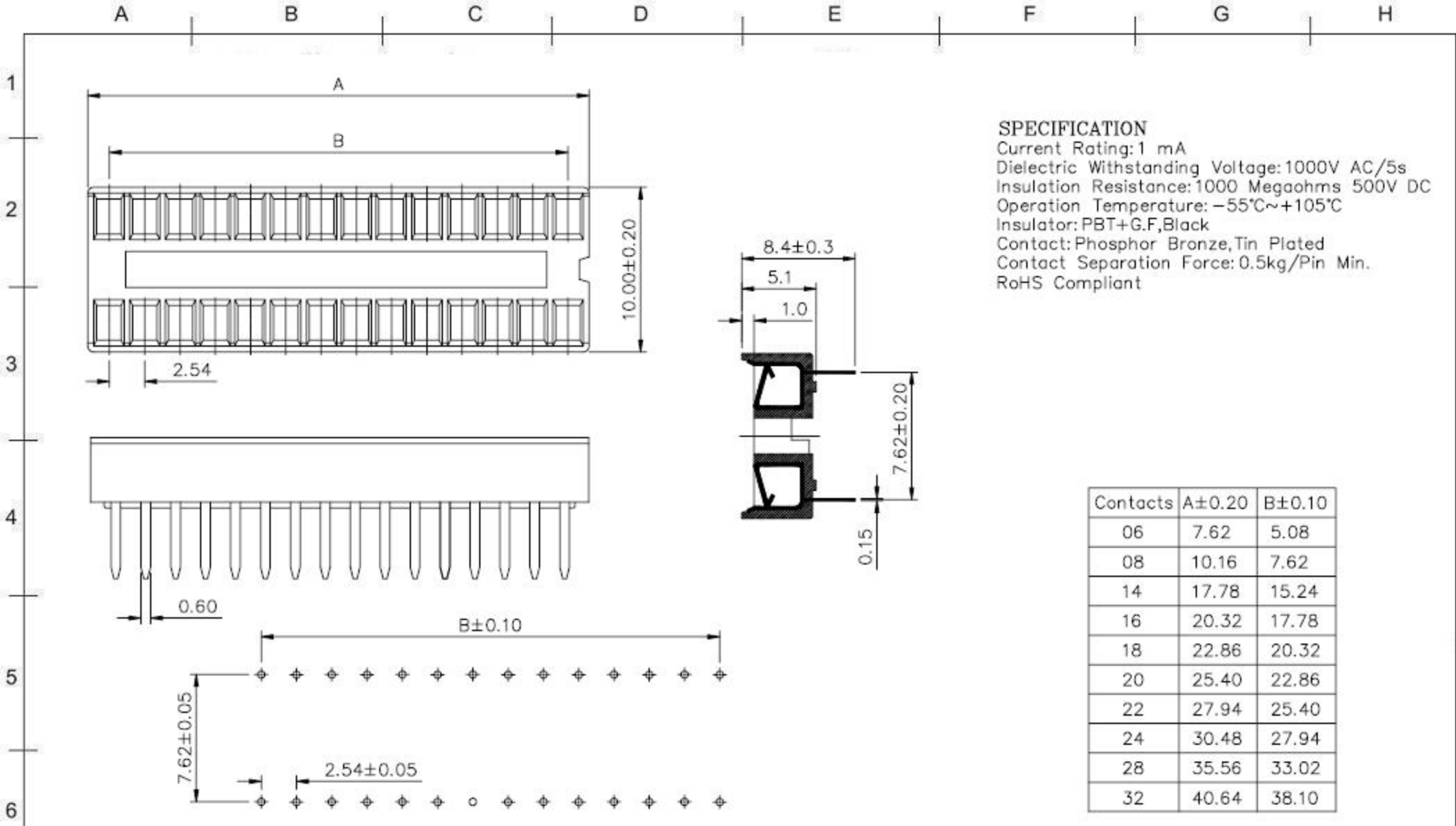
PCB Layout
