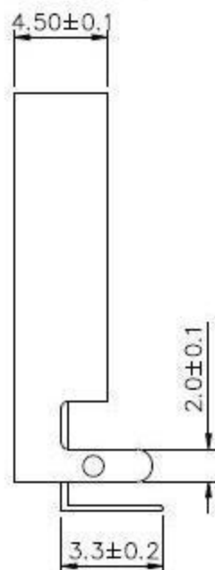
PCB Layout
